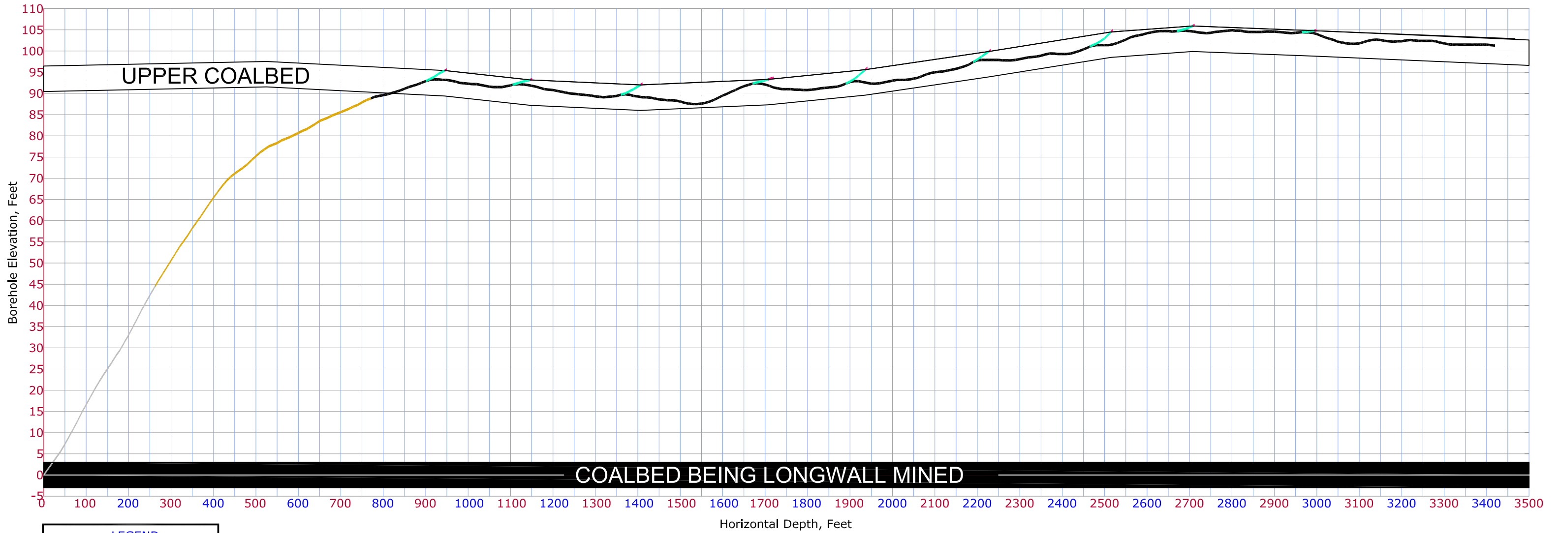
Sideview of In-Mine Borehole Targeting "Upper Coalbed"
